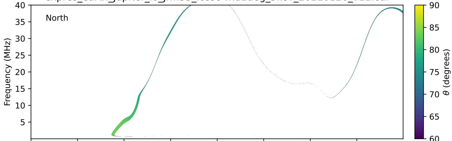
expres_earth_jupiter_io_jrm33_lossc-wid1deg_3kev_20210126_v11.cdf
