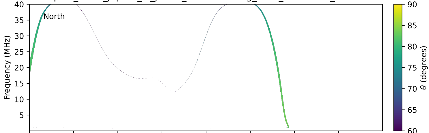
expres_earth_jupiter_io_jrm33_lossc-wid1deg_3kev_20210121_v11.cdf
