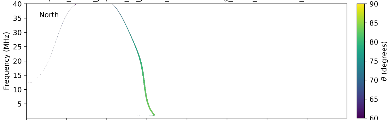
expres_earth_jupiter_io_jrm33_lossc-wid1deg_3kev_20210116_v11.cdf
