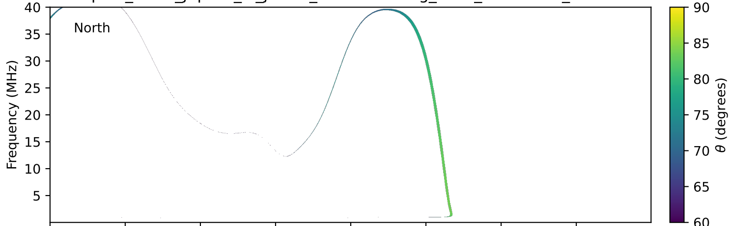
expres_earth_jupiter_io_jrm33_lossc-wid1deg_3kev_20210114_v11.cdf
