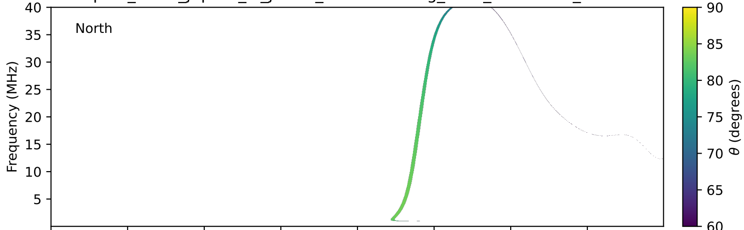
expres_earth_jupiter_io_jrm33_lossc-wid1deg_3kev_20210108_v11.cdf
