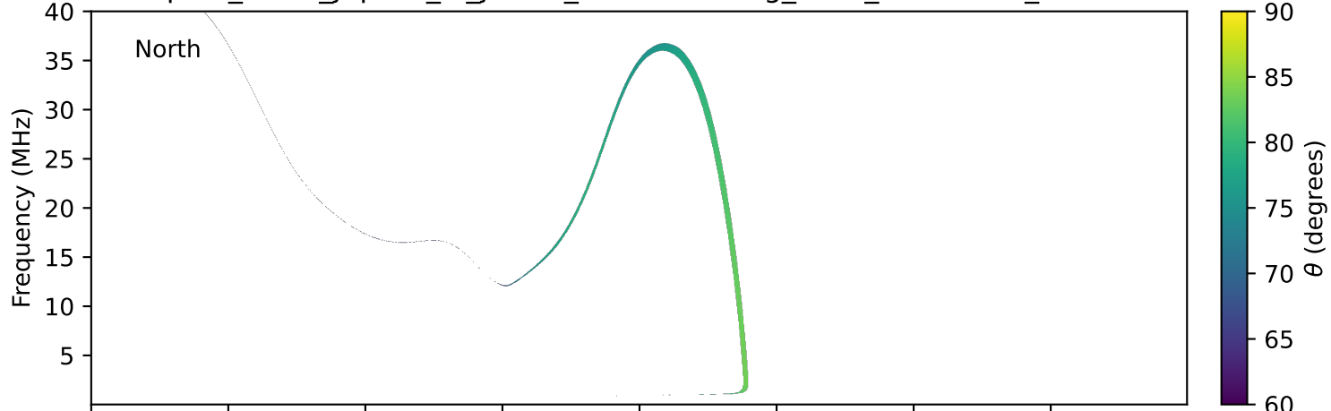
expres_earth_jupiter_io_jrm33_lossc-wid1deg_3kev_20210107_v11.cdf
