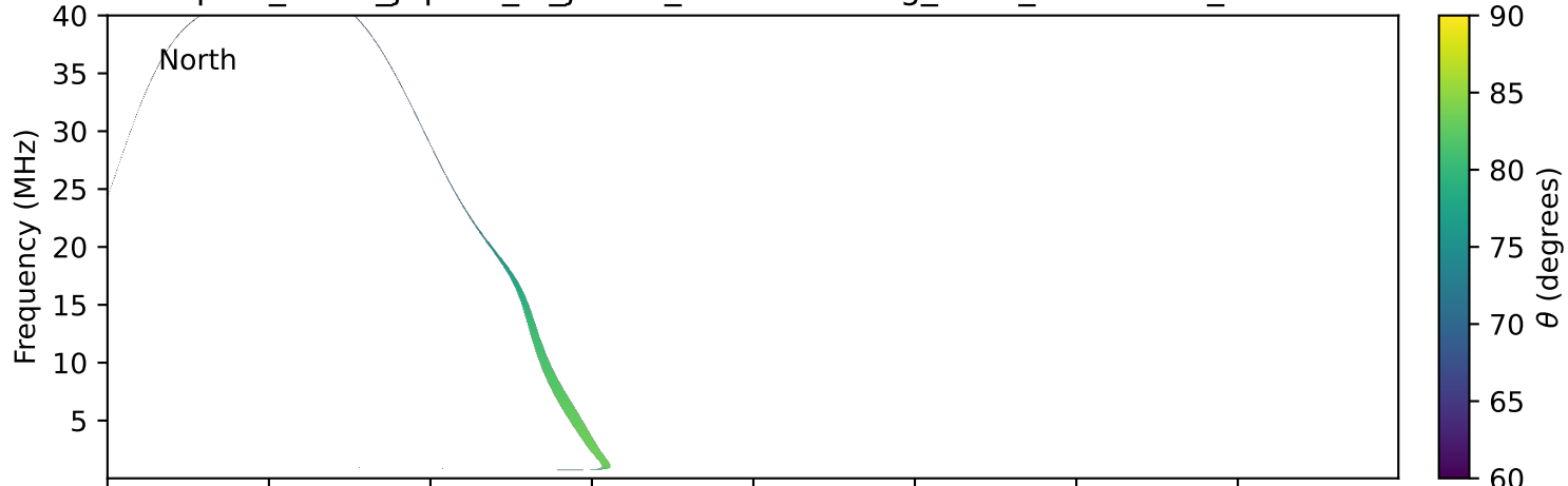
expres_earth_jupiter_io_jrm33_lossc-wid1deg_3kev_20210102_v11.cdf
