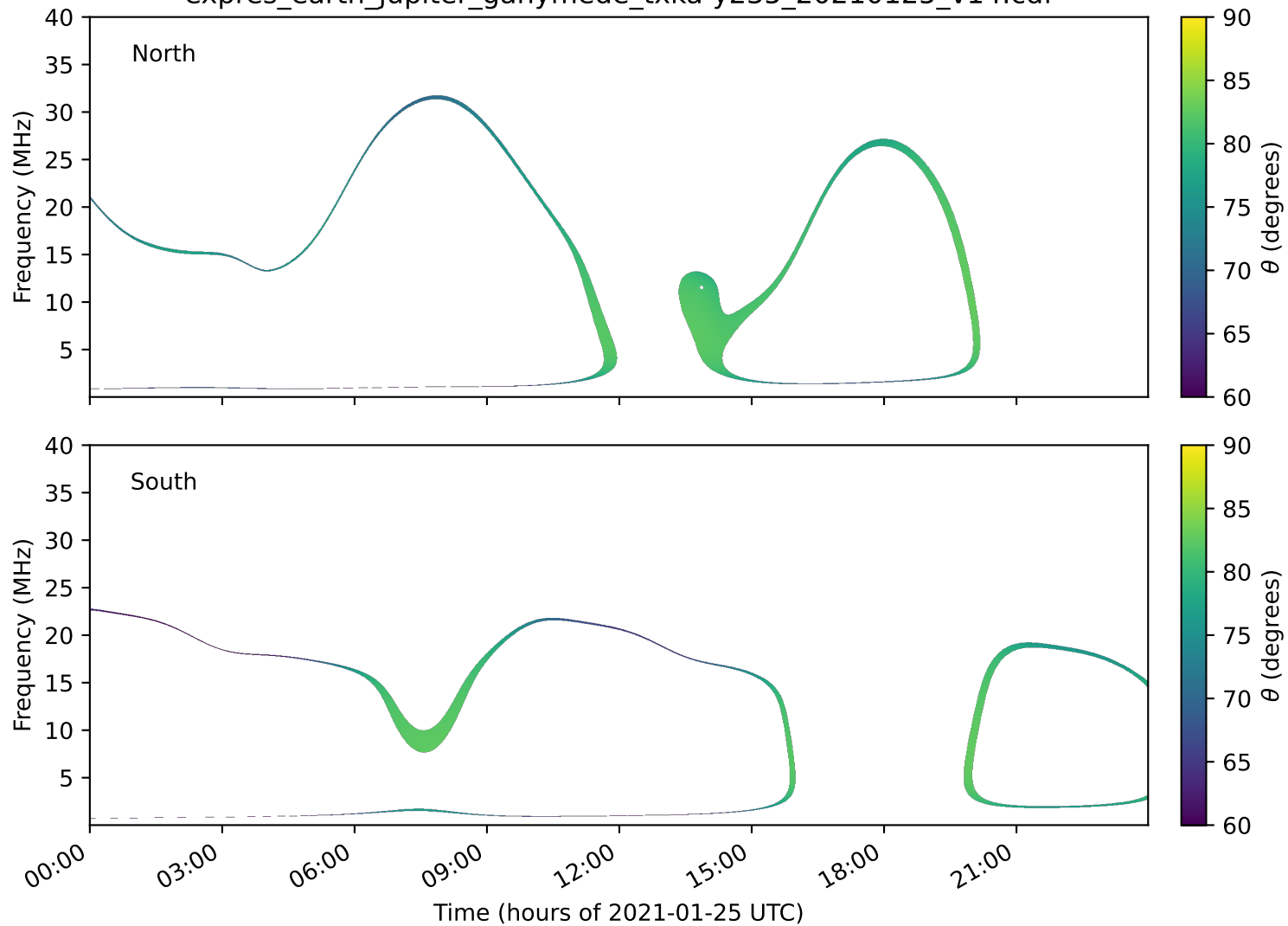
expres_earth_jupiter_ganymede_txka-y235_20210125_v14.cdf
