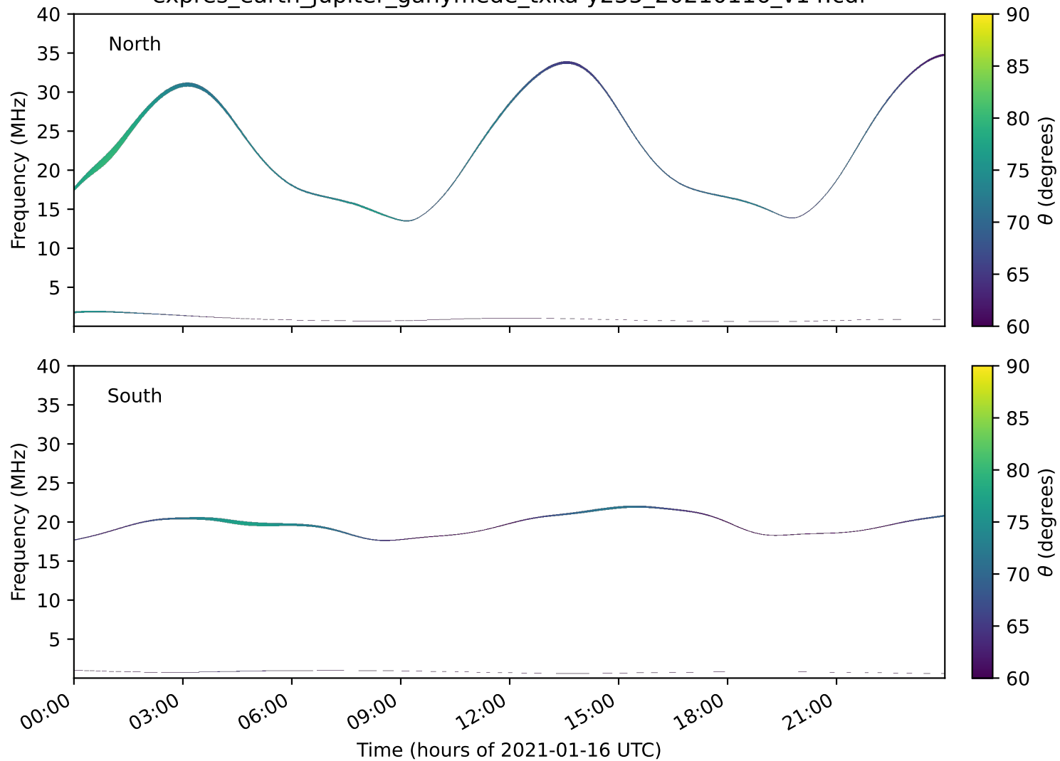
expres_earth_jupiter_ganymede_txka-y235_20210116_v14.cdf
