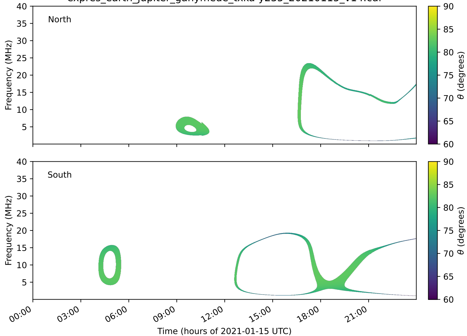
expres_earth_jupiter_ganymede_txka-y235_20210115_v14.cdf
