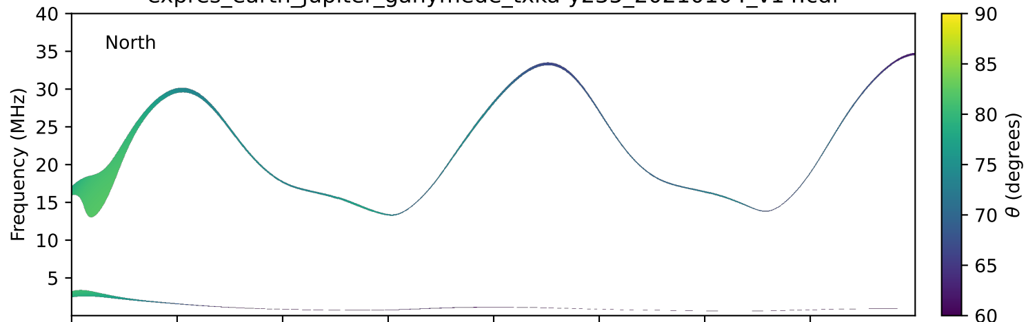
expres_earth_jupiter_ganymede_txka-y235_20210104_v14.cdf
