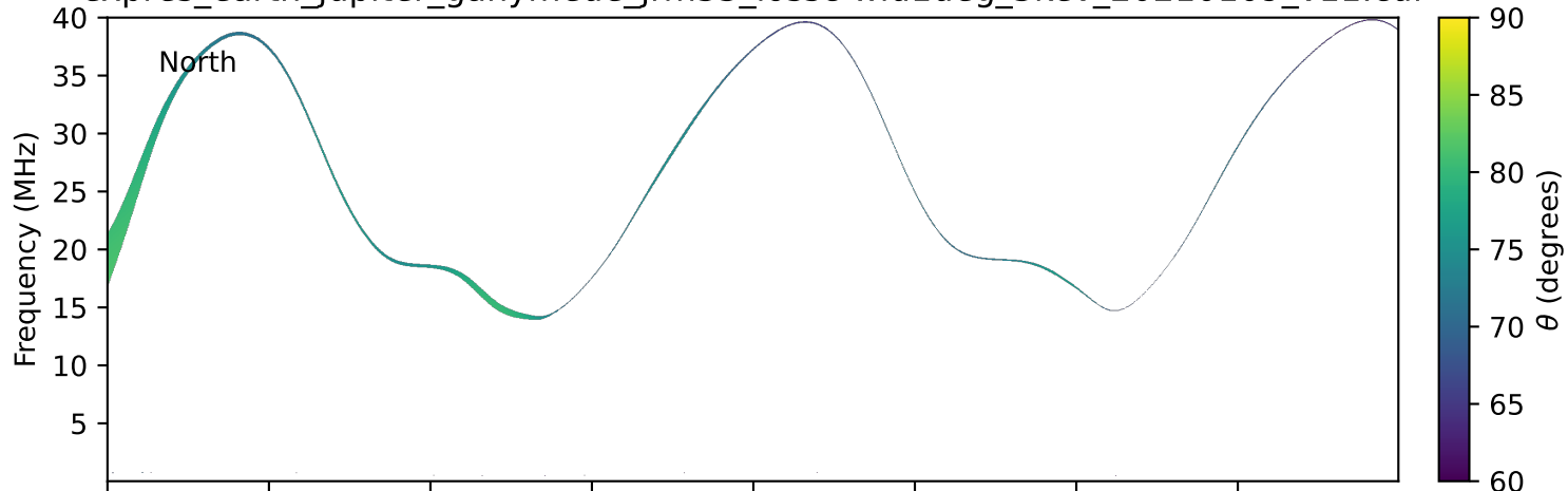
expres_earth_jupiter_ganymede_jrm33_lossc-wid1deg_3kev_20210109_v11.cdf
