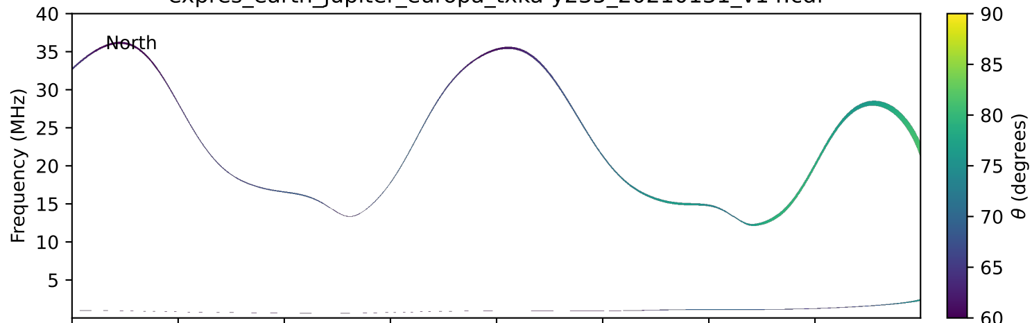
expres_earth_jupiter_europa_txka-y235_20210131_v14.cdf
