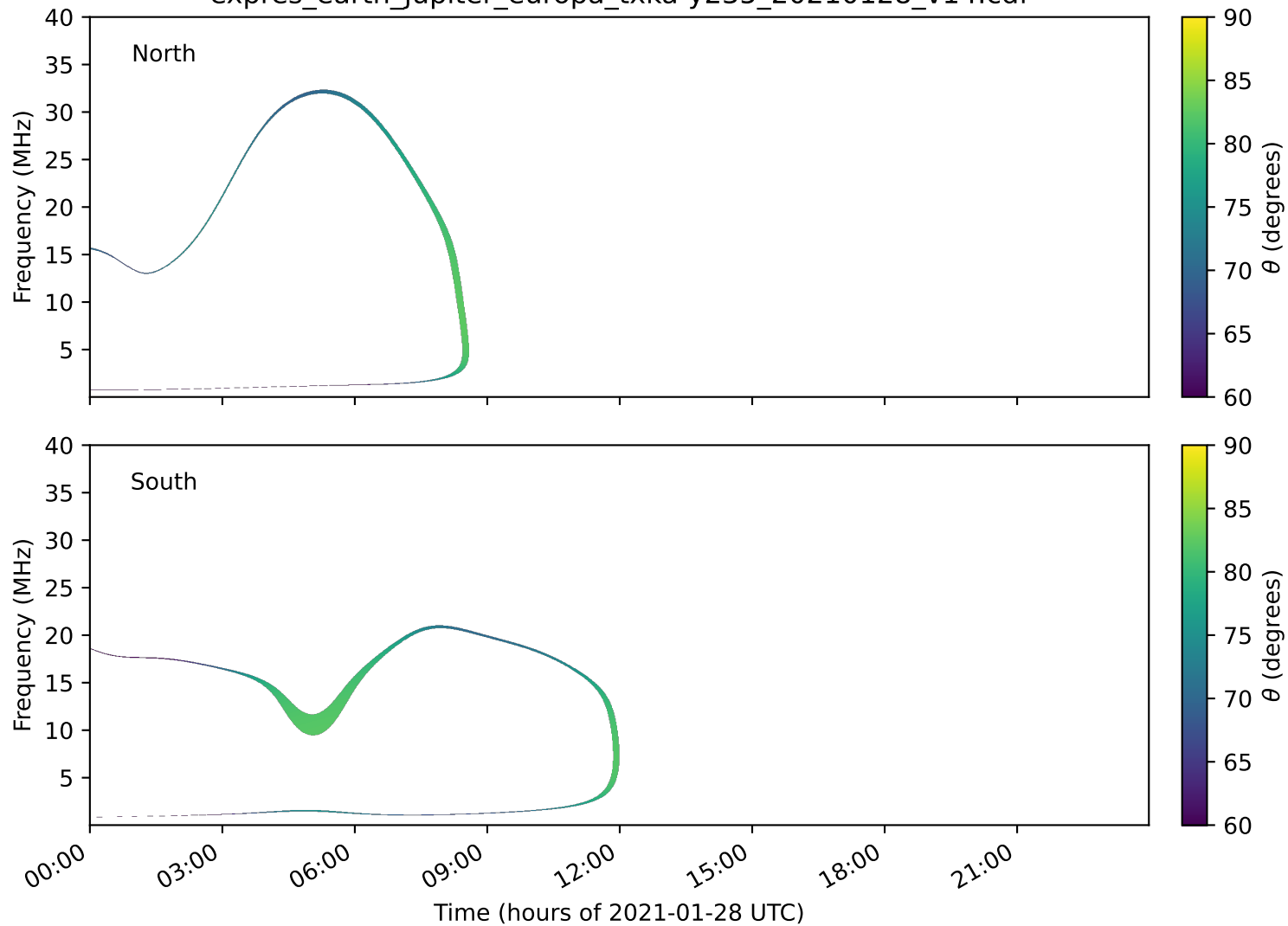
expres_earth_jupiter_europa_txka-y235_20210128_v14.cdf
