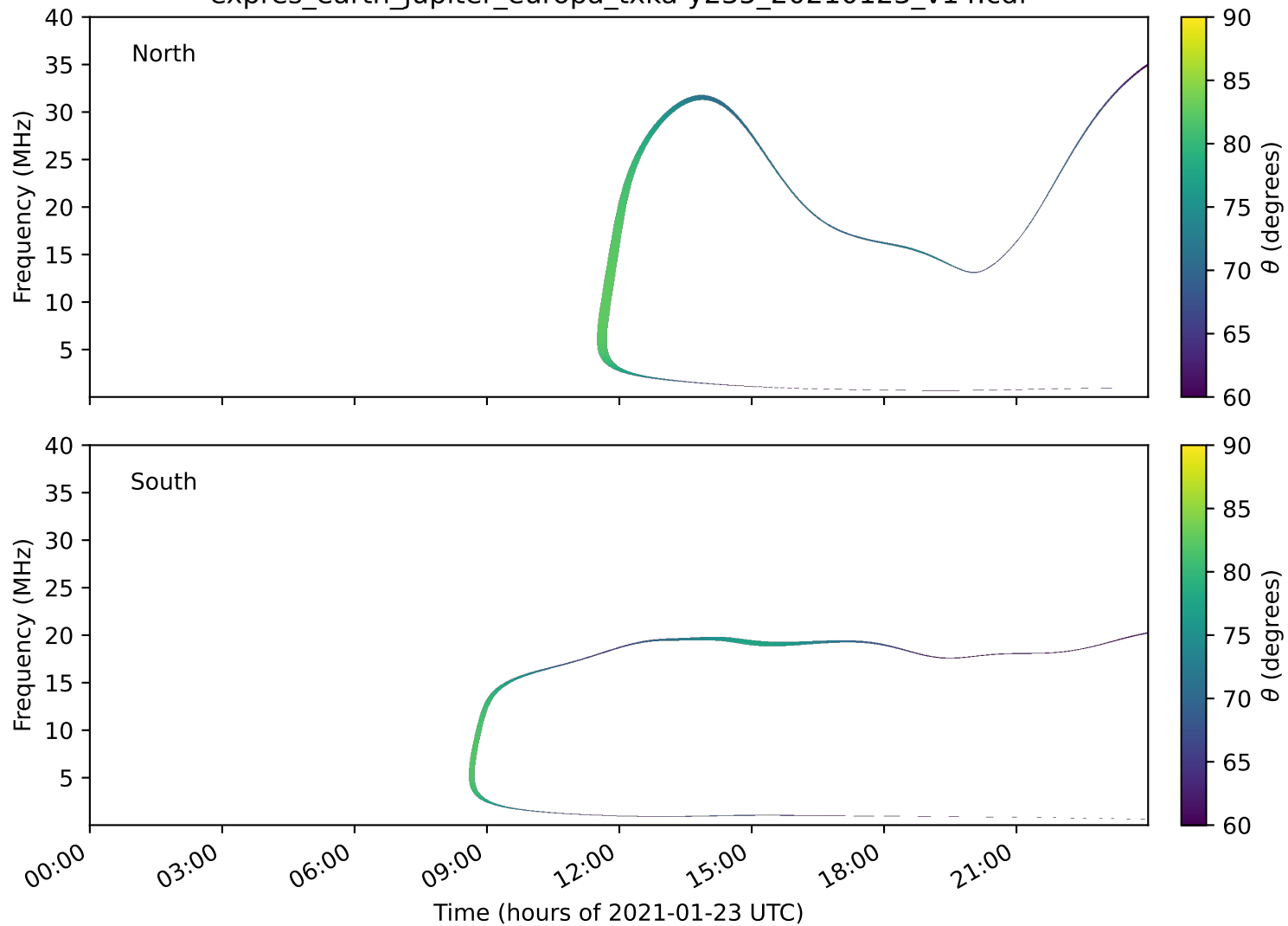
expres_earth_jupiter_europa_txka-y235_20210123_v14.cdf
