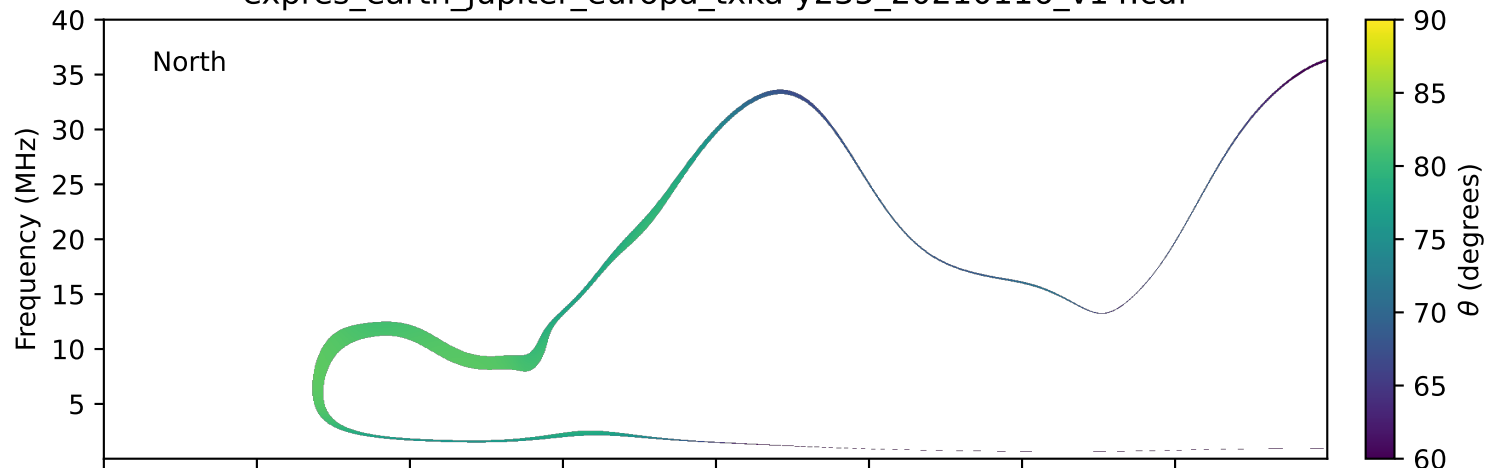
expres_earth_jupiter_europa_txka-y235_20210116_v14.cdf
