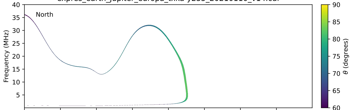
expres_earth_jupiter_europa_txka-y235_20210110_v14.cdf
