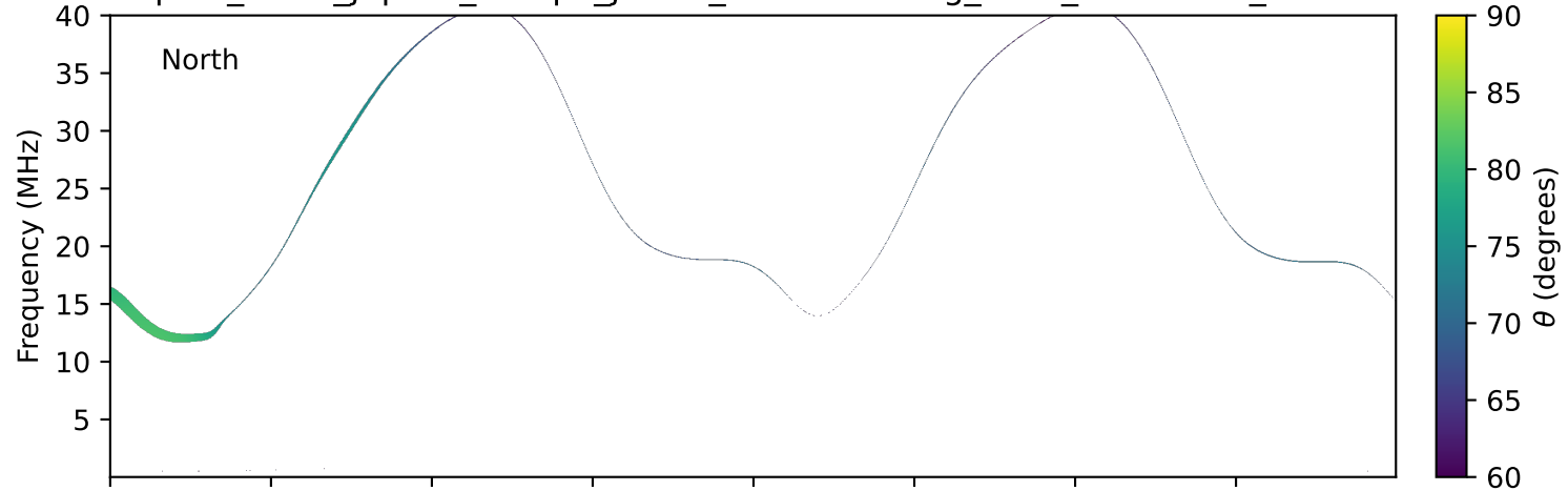
expres_earth_jupiter_europa_jrm33_lossc-wid1deg_3kev_20210120_v11.cdf
