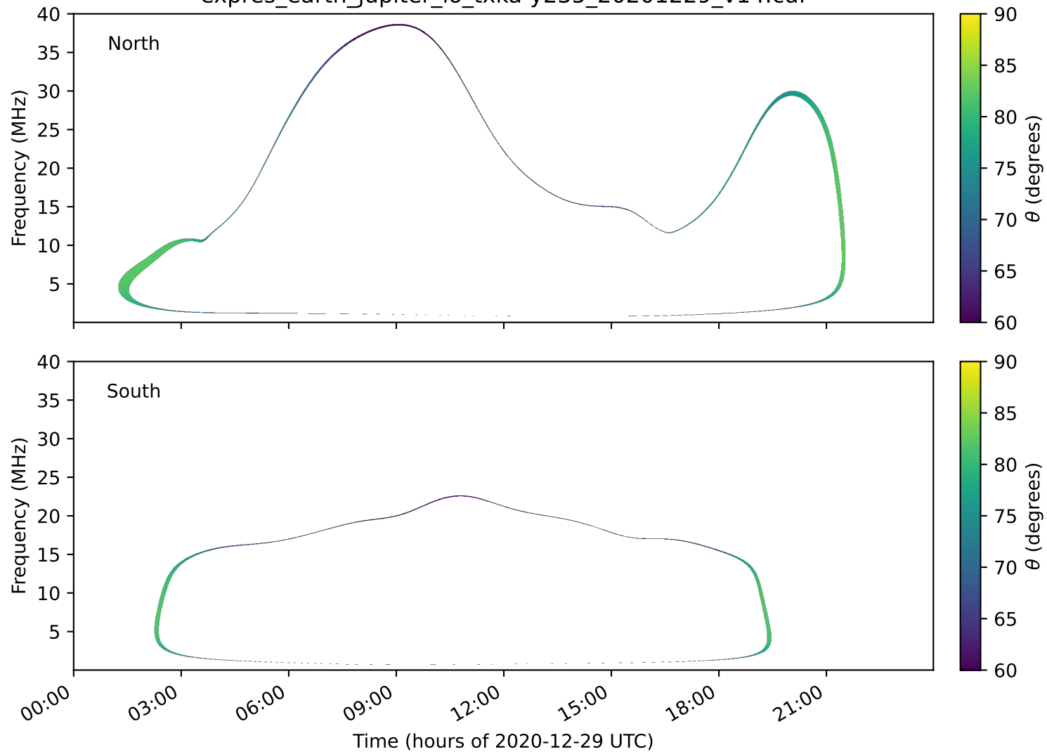
expres_earth_jupiter_io_txka-y235_20201229_v14.cdf
