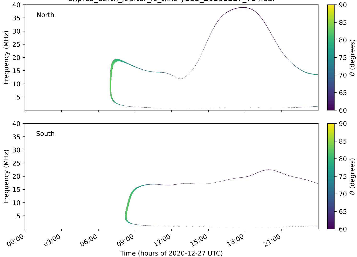
expres_earth_jupiter_io_txka-y235_20201227_v14.cdf
