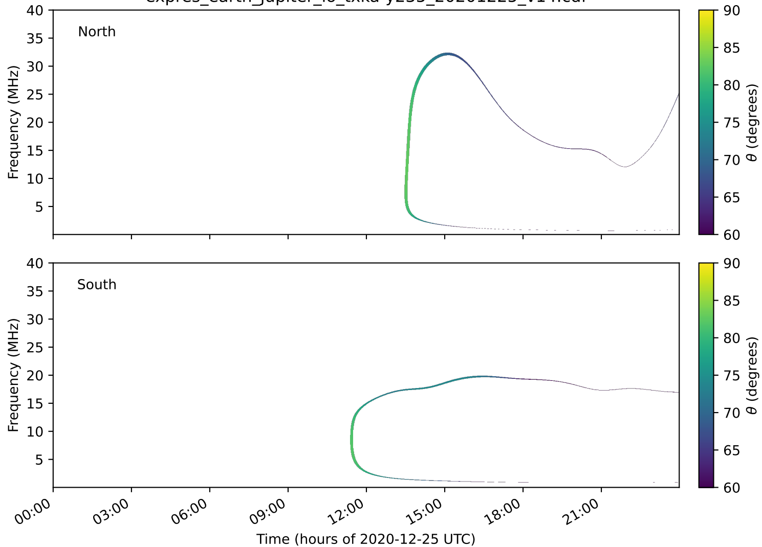
expres_earth_jupiter_io_txka-y235_20201225_v14.cdf
