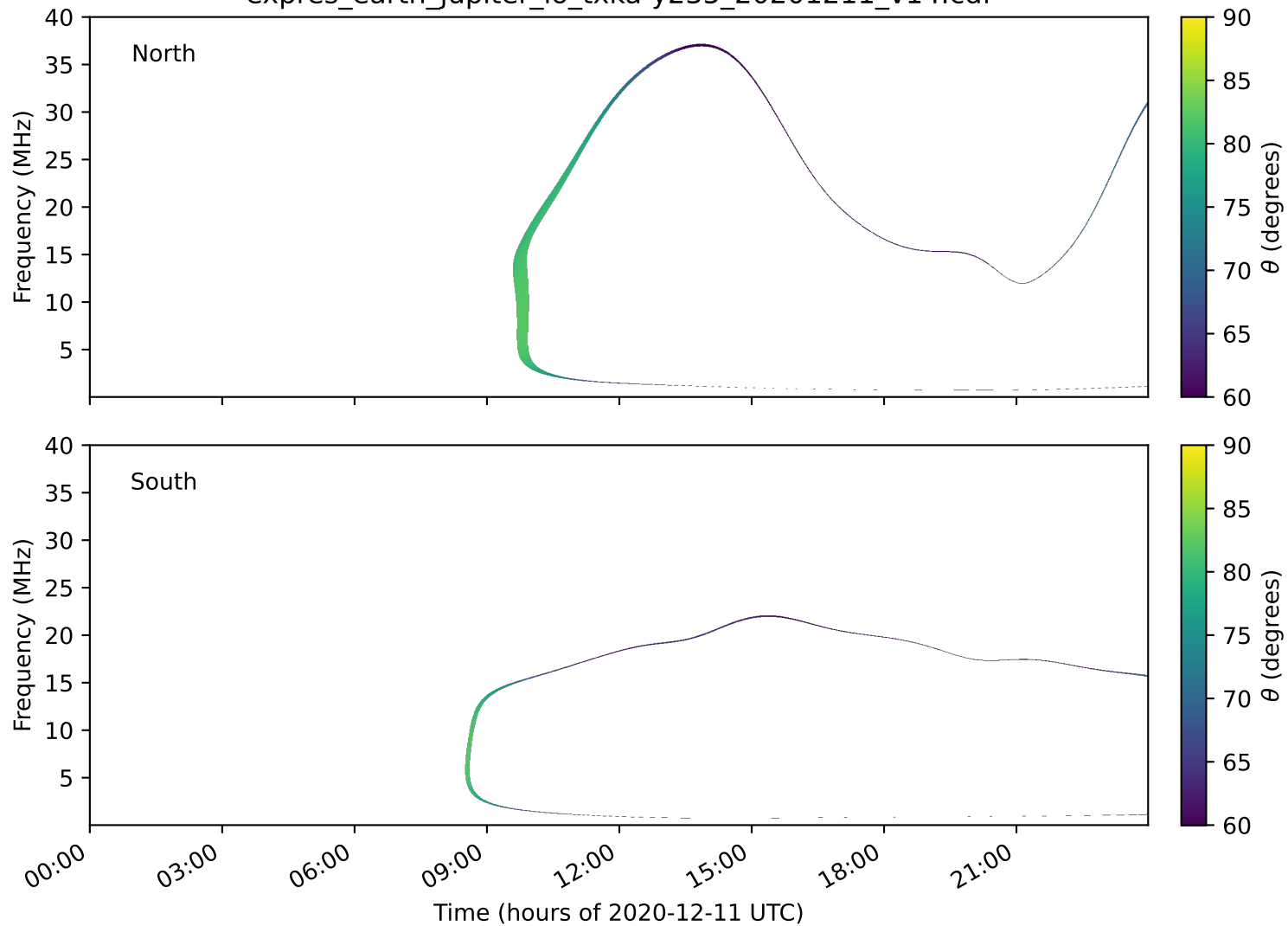
expres_earth_jupiter_io_txka-y235_20201211_v14.cdf
