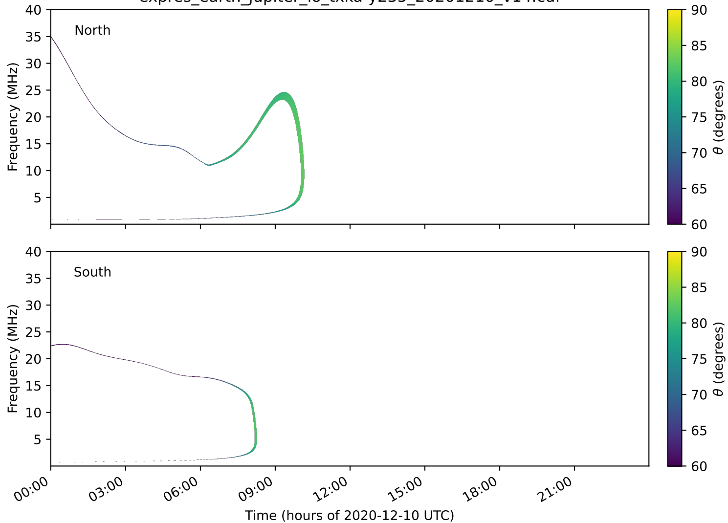
expres_earth_jupiter_io_txka-y235_20201210_v14.cdf
