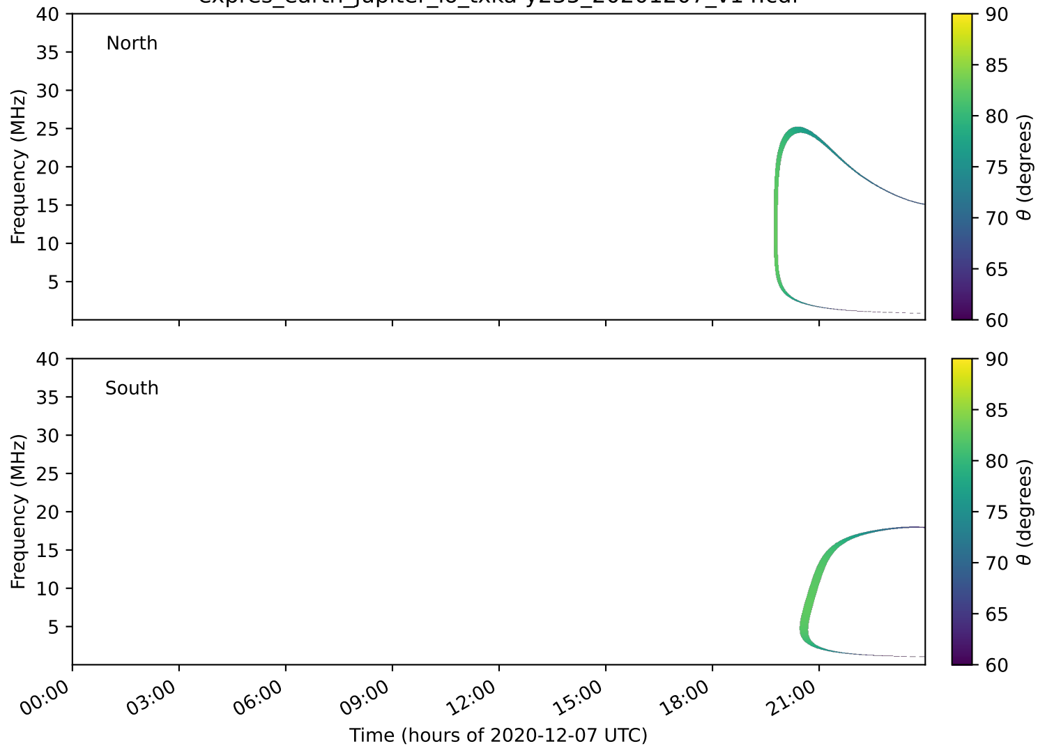
expres_earth_jupiter_io_txka-y235_20201207_v14.cdf
