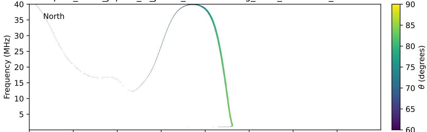
expres_earth_jupiter_io_jrm33_lossc-wid1deg_3kev_20201224_v11.cdf
