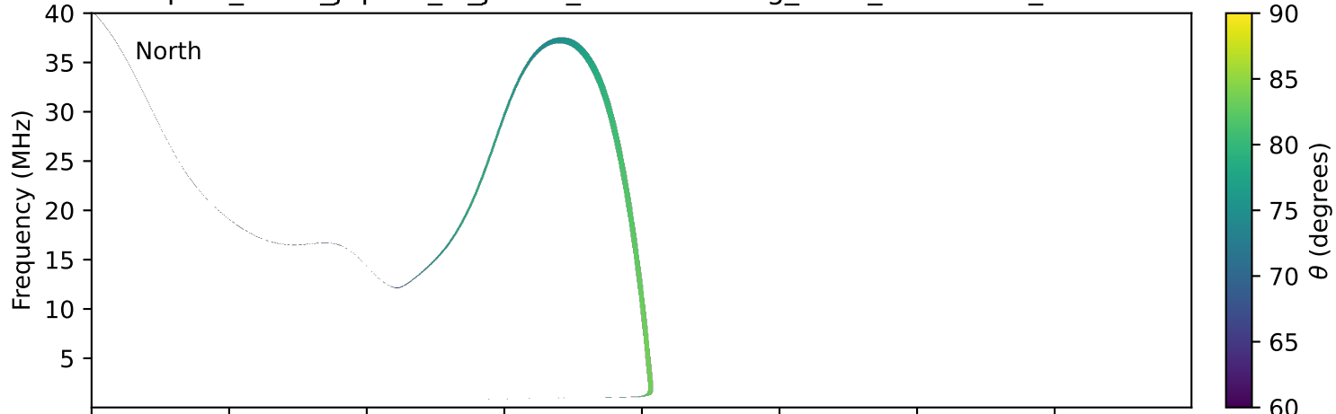
expres_earth_jupiter_io_jrm33_lossc-wid1deg_3kev_20201217_v11.cdf
