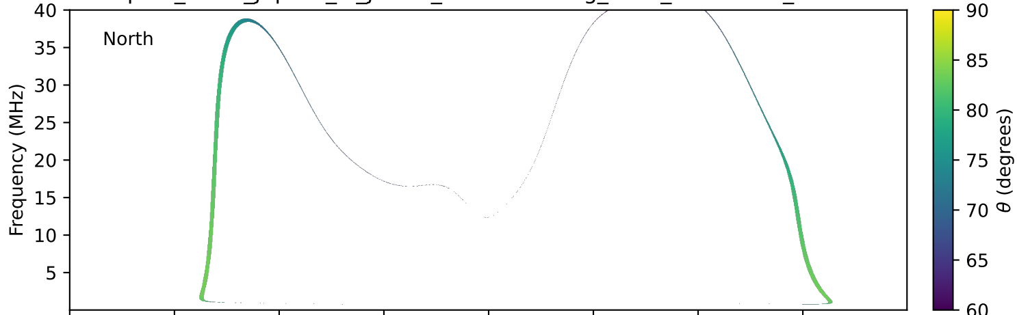
expres_earth_jupiter_io_jrm33_lossc-wid1deg_3kev_20201213_v11.cdf
