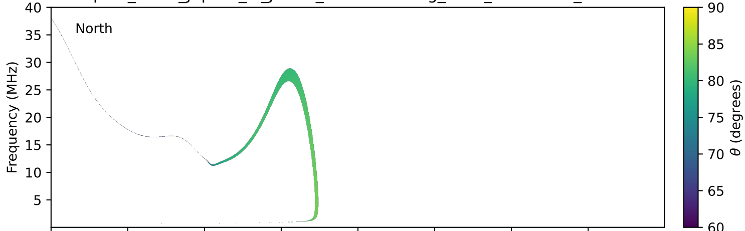
expres_earth_jupiter_io_jrm33_lossc-wid1deg_3kev_20201210_v11.cdf
