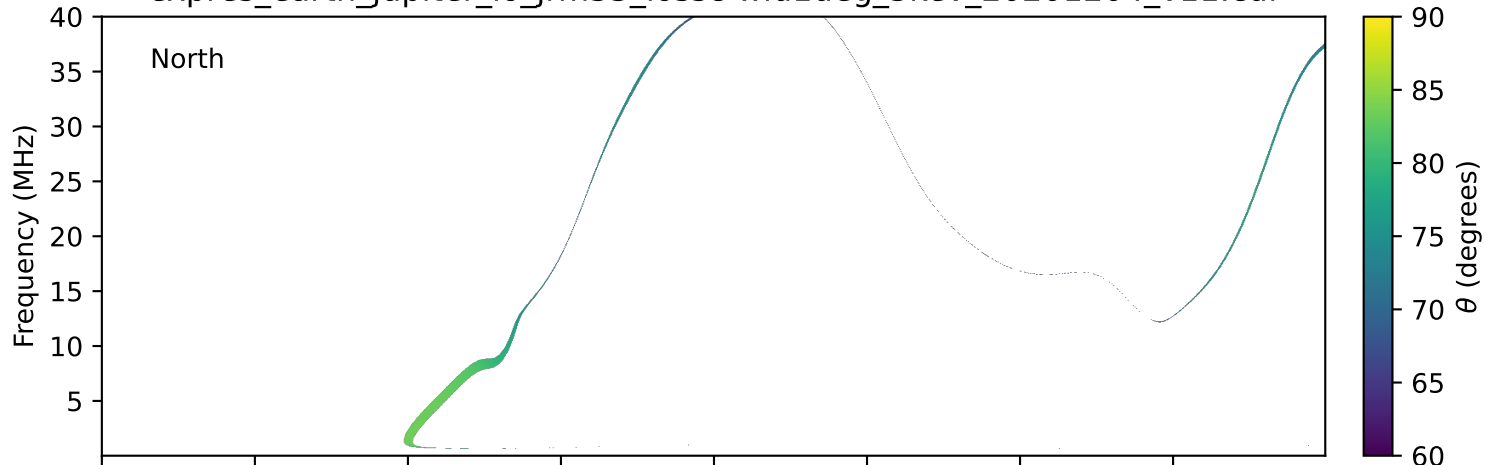
expres_earth_jupiter_io_jrm33_lossc-wid1deg_3kev_20201204_v11.cdf
