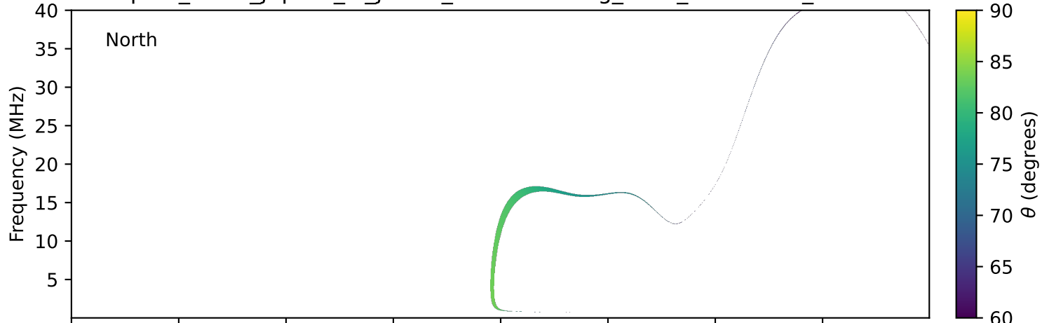
expres_earth_jupiter_io_jrm33_lossc-wid1deg_3kev_20201202_v11.cdf
