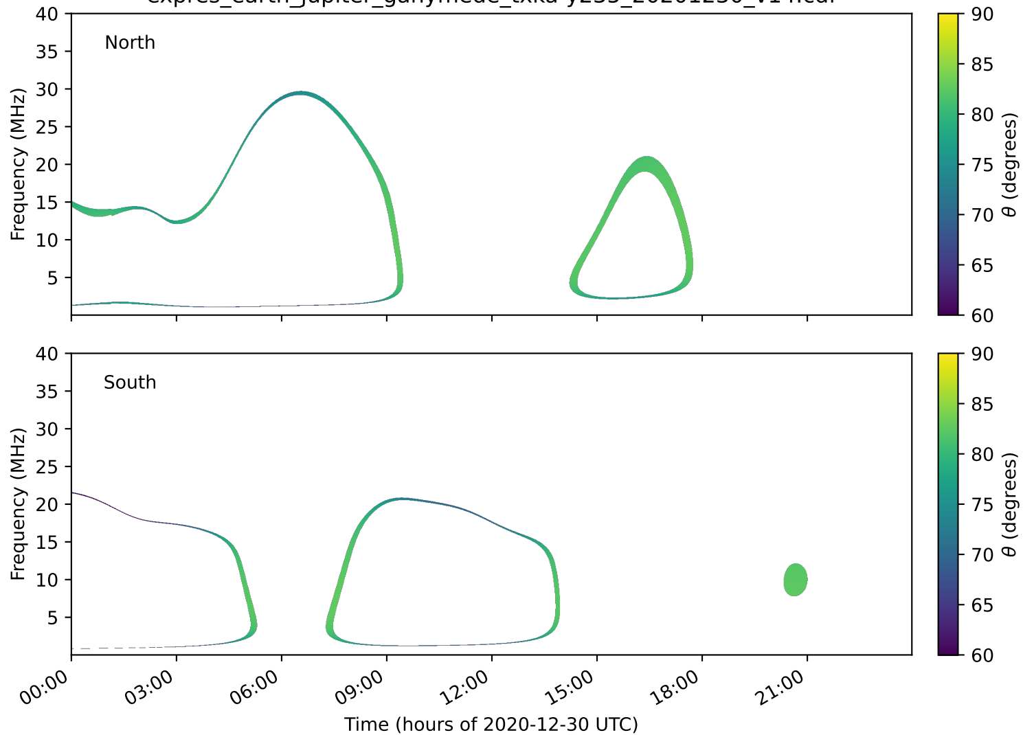
expres_earth_jupiter_ganymede_txka-y235_20201230_v14.cdf
