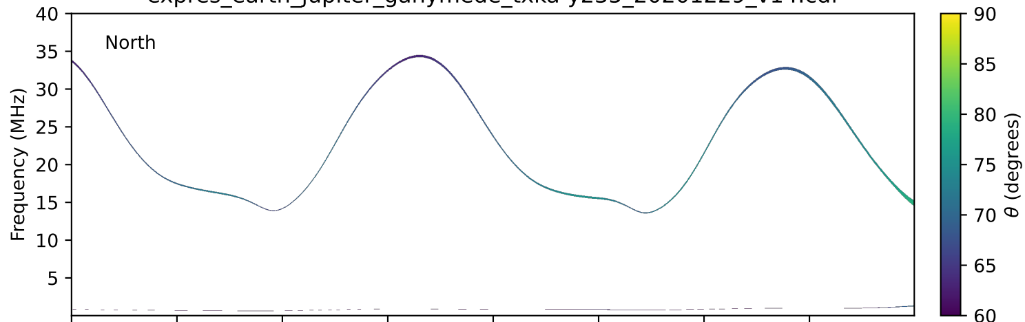
expres_earth_jupiter_ganymede_txka-y235_20201229_v14.cdf
