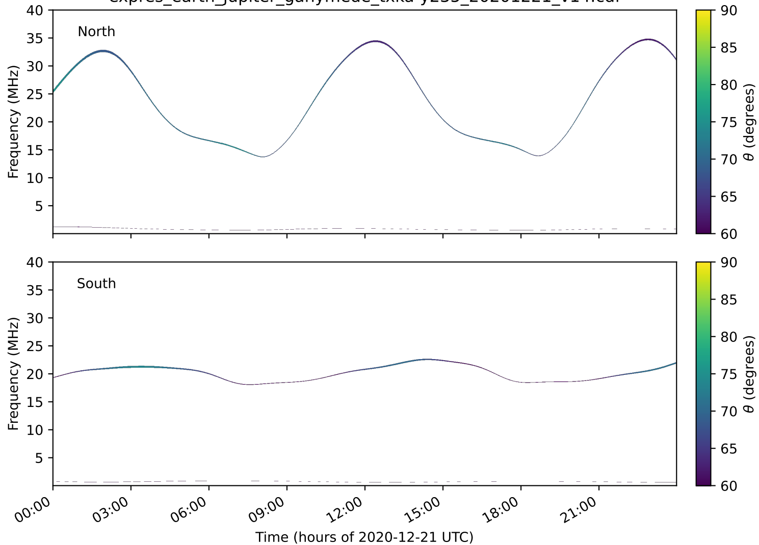
expres_earth_jupiter_ganymede_txka-y235_20201221_v14.cdf
