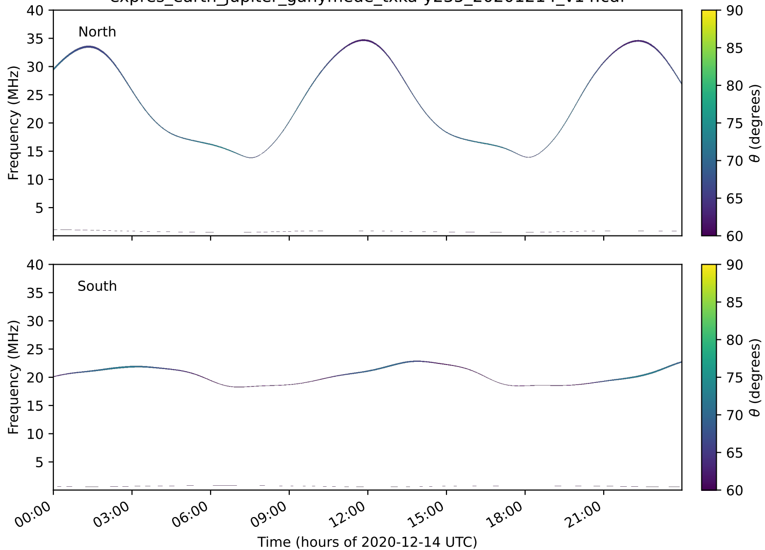
expres_earth_jupiter_ganymede_txka-y235_20201214_v14.cdf
