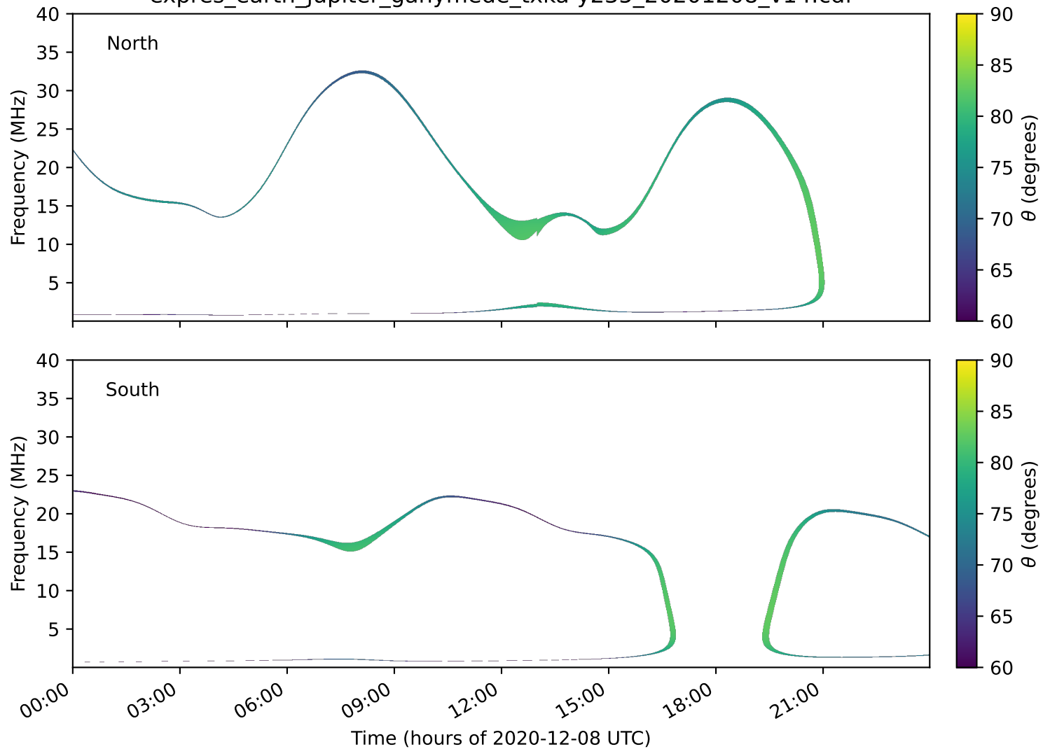
expres_earth_jupiter_ganymede_txka-y235_20201208_v14.cdf
