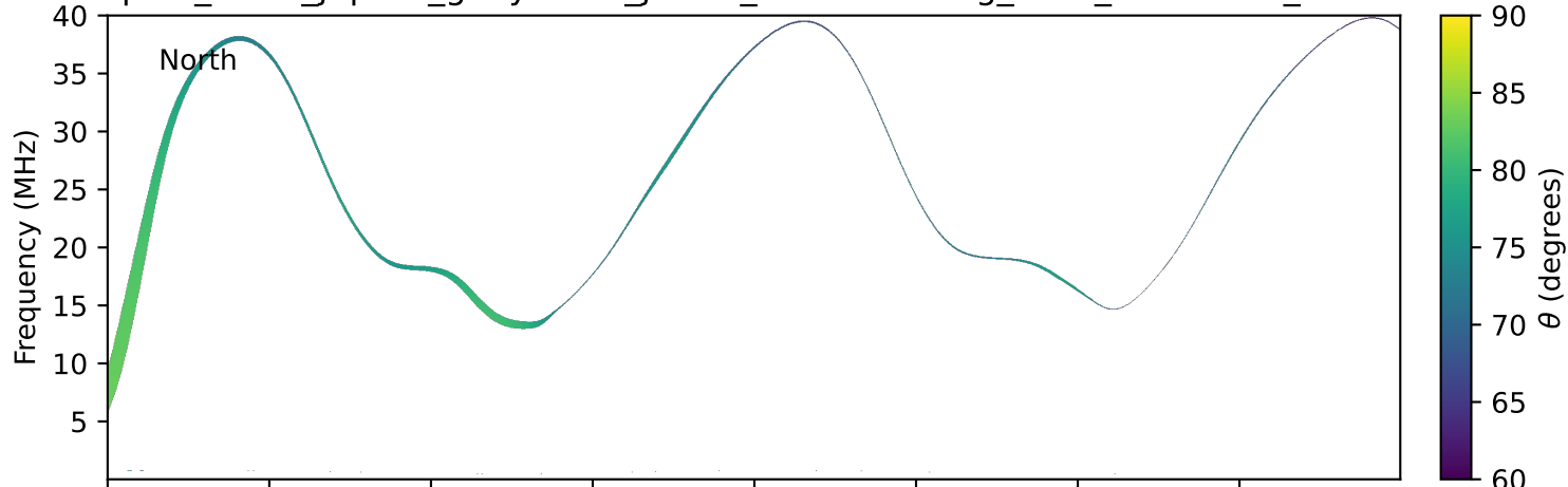
expres_earth_jupiter_ganymede_jrm33_lossc-wid1deg_3kev_20201228_v11.cdf
