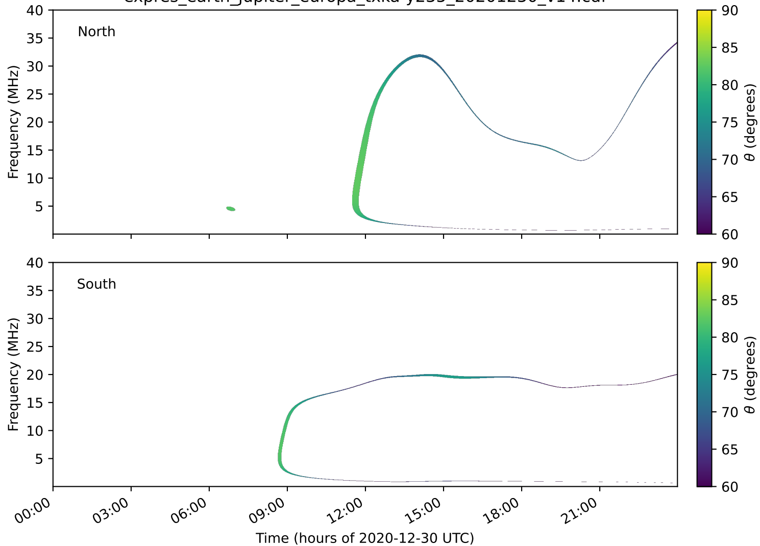
expres_earth_jupiter_europa_txka-y235_20201230_v14.cdf
