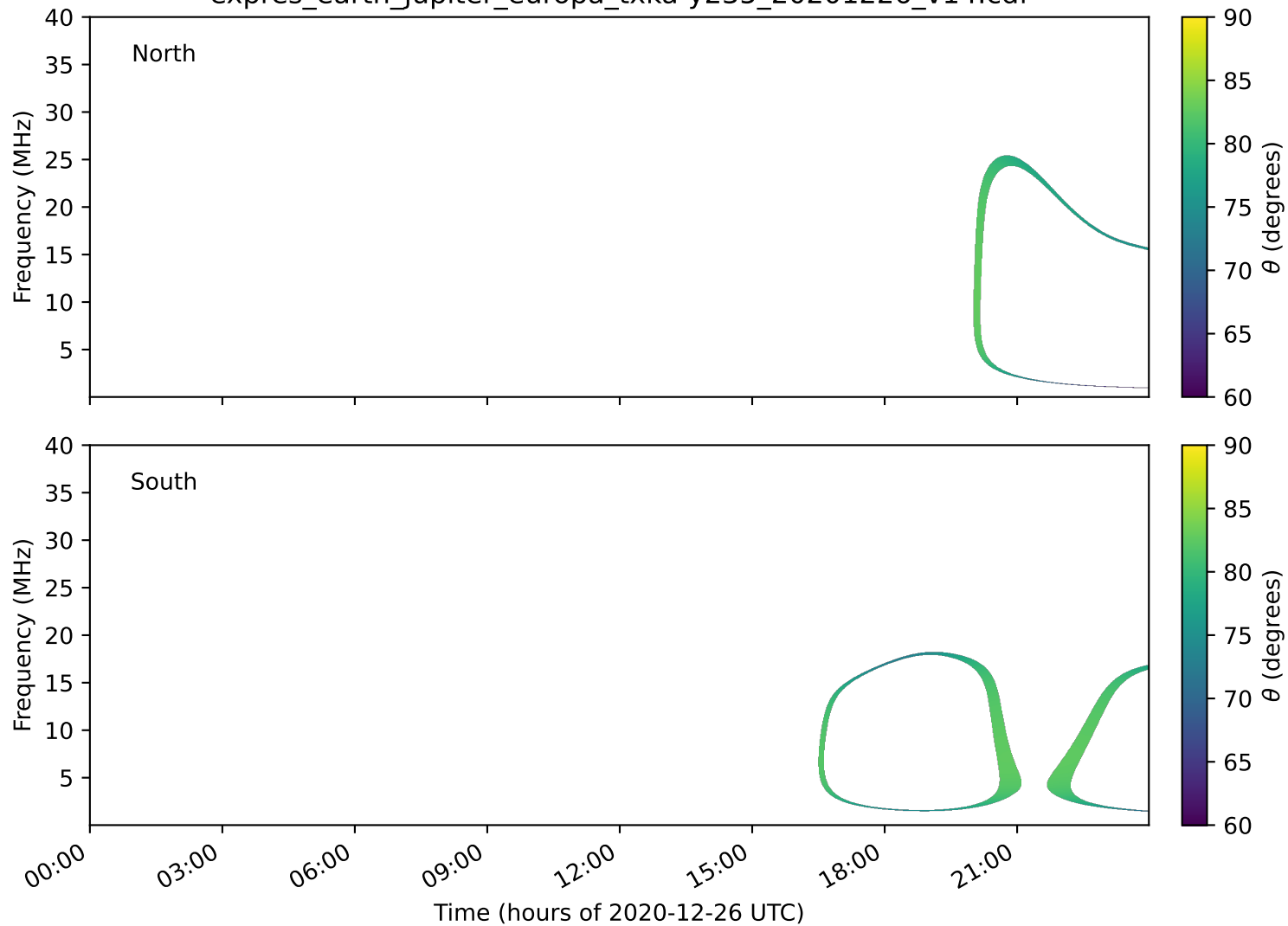
expres_earth_jupiter_europa_txka-y235_20201226_v14.cdf
