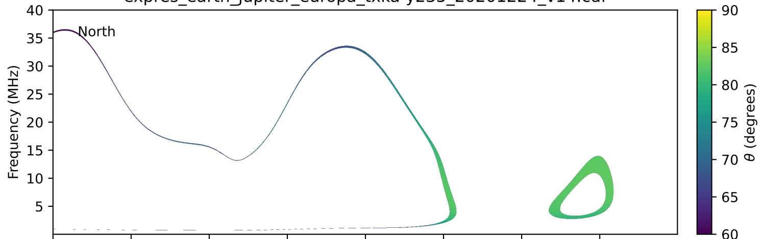
expres_earth_jupiter_europa_txka-y235_20201224_v14.cdf
