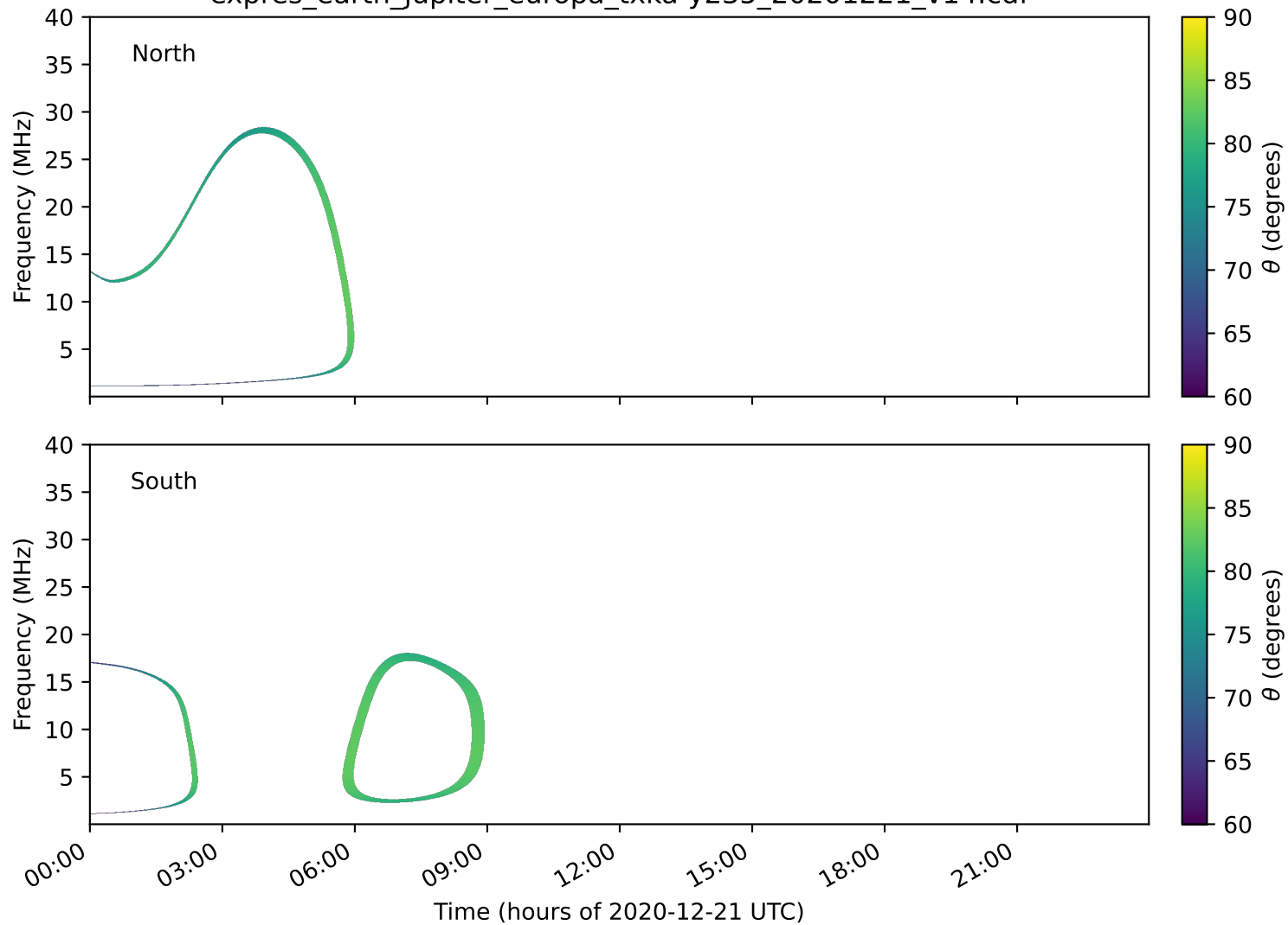
expres_earth_jupiter_europa_txka-y235_20201221_v14.cdf
