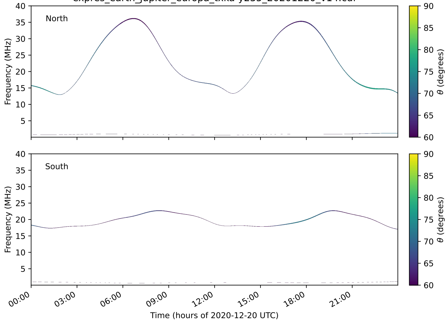
expres_earth_jupiter_europa_txka-y235_20201220_v14.cdf
