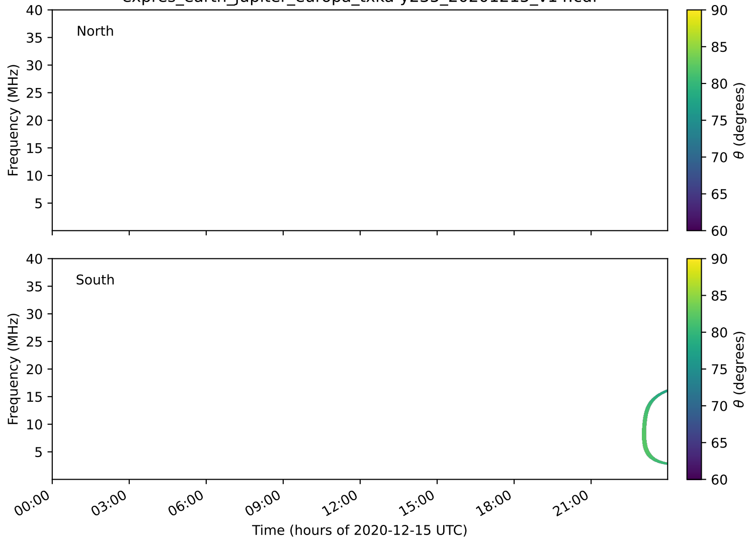
expres_earth_jupiter_europa_txka-y235_20201215_v14.cdf
