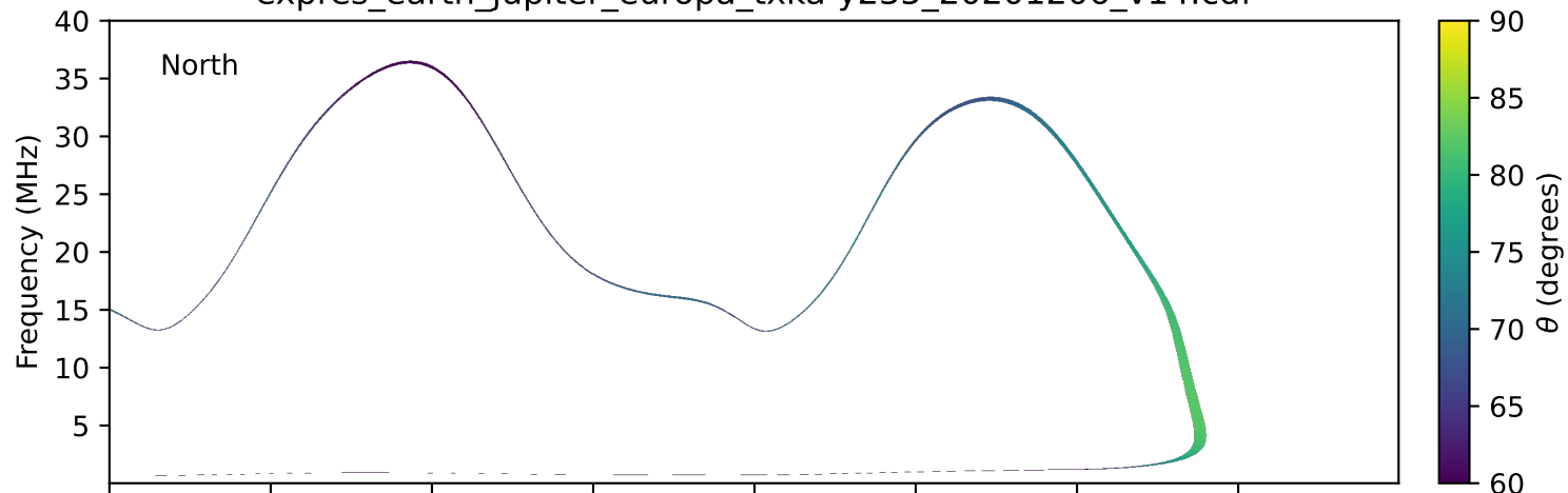
expres_earth_jupiter_europa_txka-y235_20201206_v14.cdf
