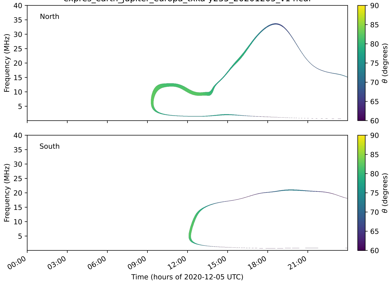
expres_earth_jupiter_europa_txka-y235_20201205_v14.cdf
