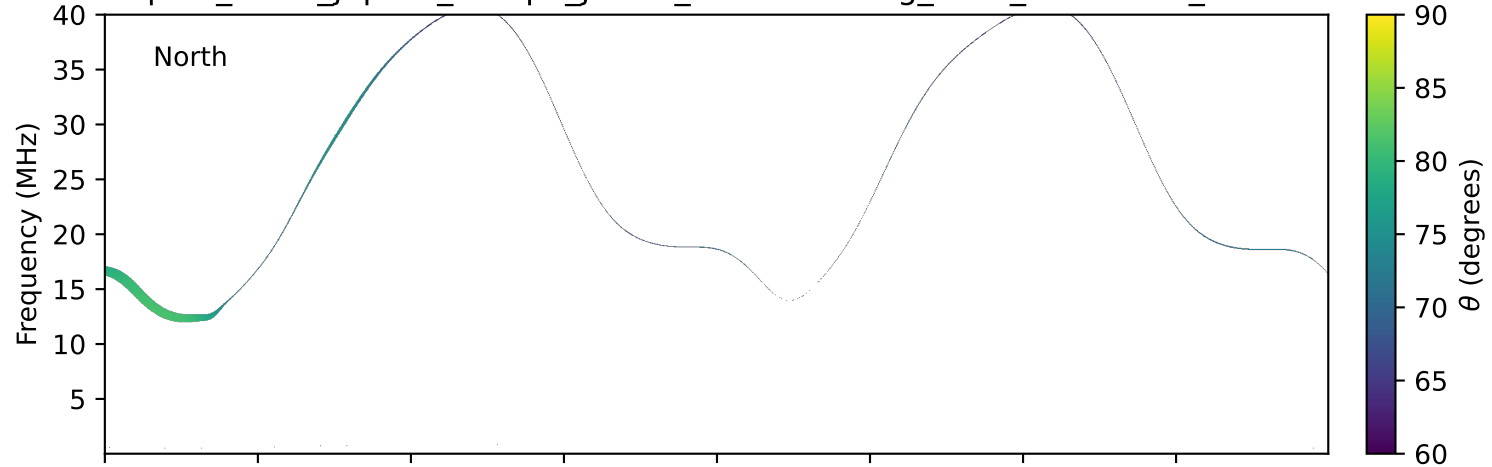
expres_earth_jupiter_europa_jrm33_lossc-wid1deg_3kev_20201227_v11.cdf
