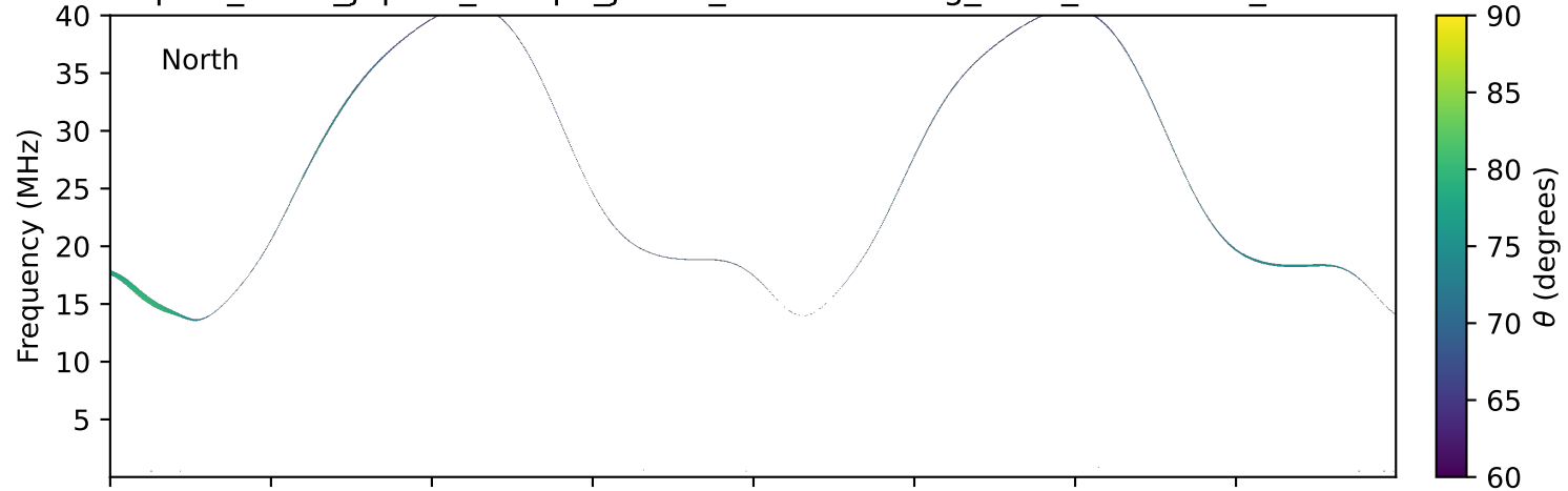
expres_earth_jupiter_europa_jrm33_lossc-wid1deg_3kev_20201220_v11.cdf
