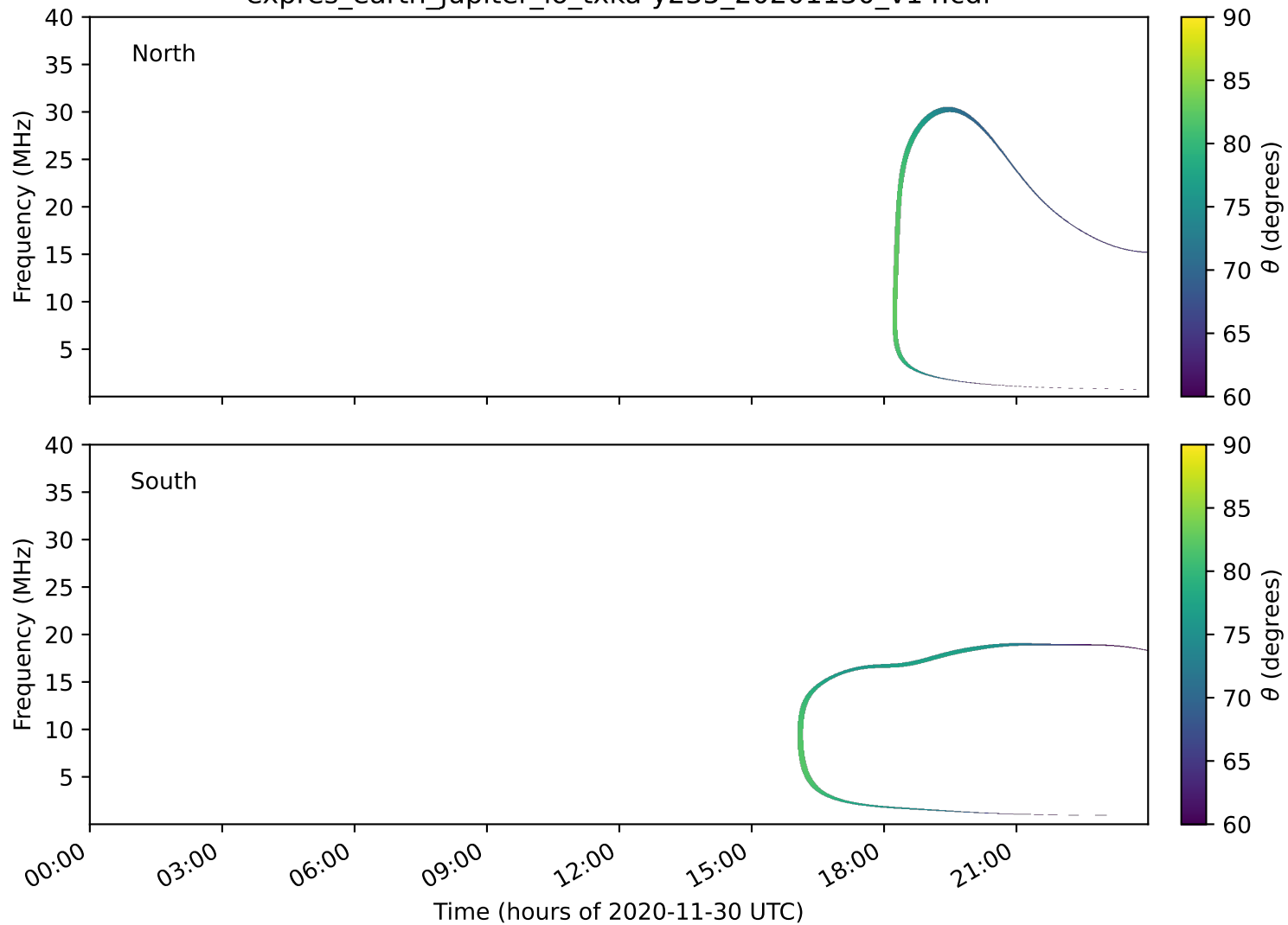
expres_earth_jupiter_io_txka-y235_20201130_v14.cdf
