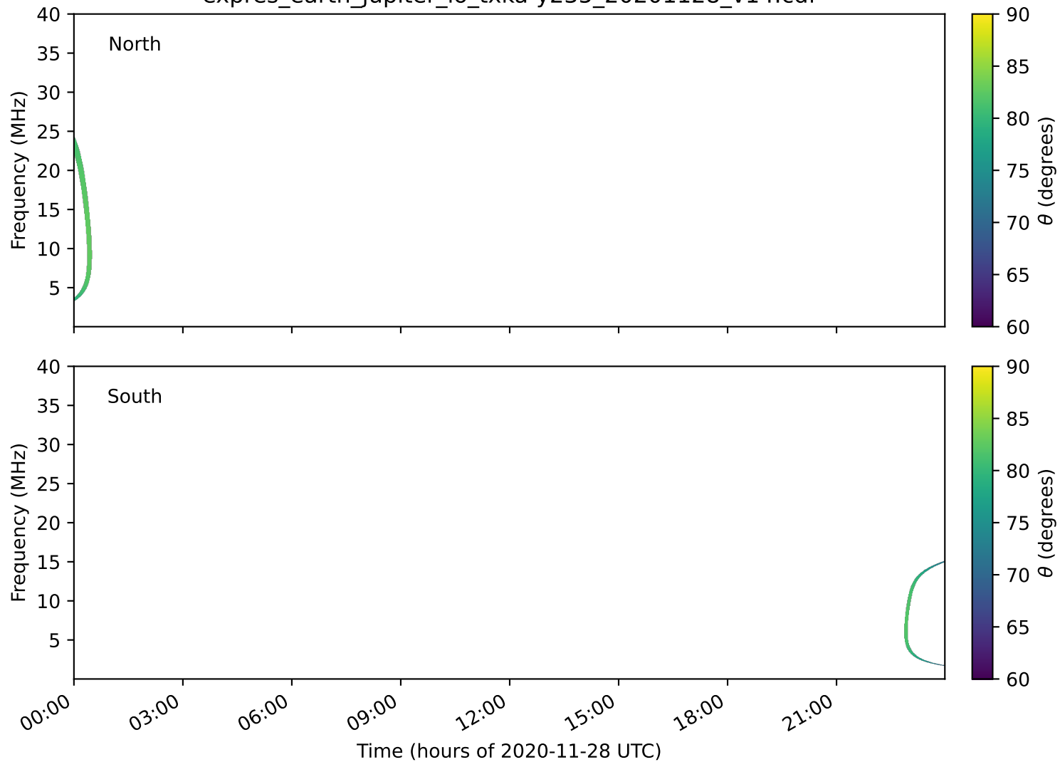
expres_earth_jupiter_io_txka-y235_20201128_v14.cdf
