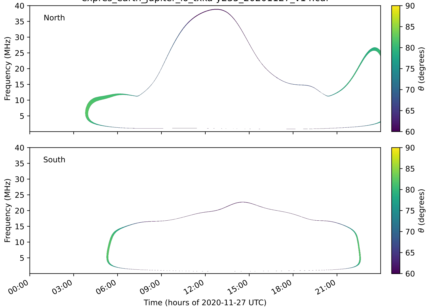
expres_earth_jupiter_io_txka-y235_20201127_v14.cdf
