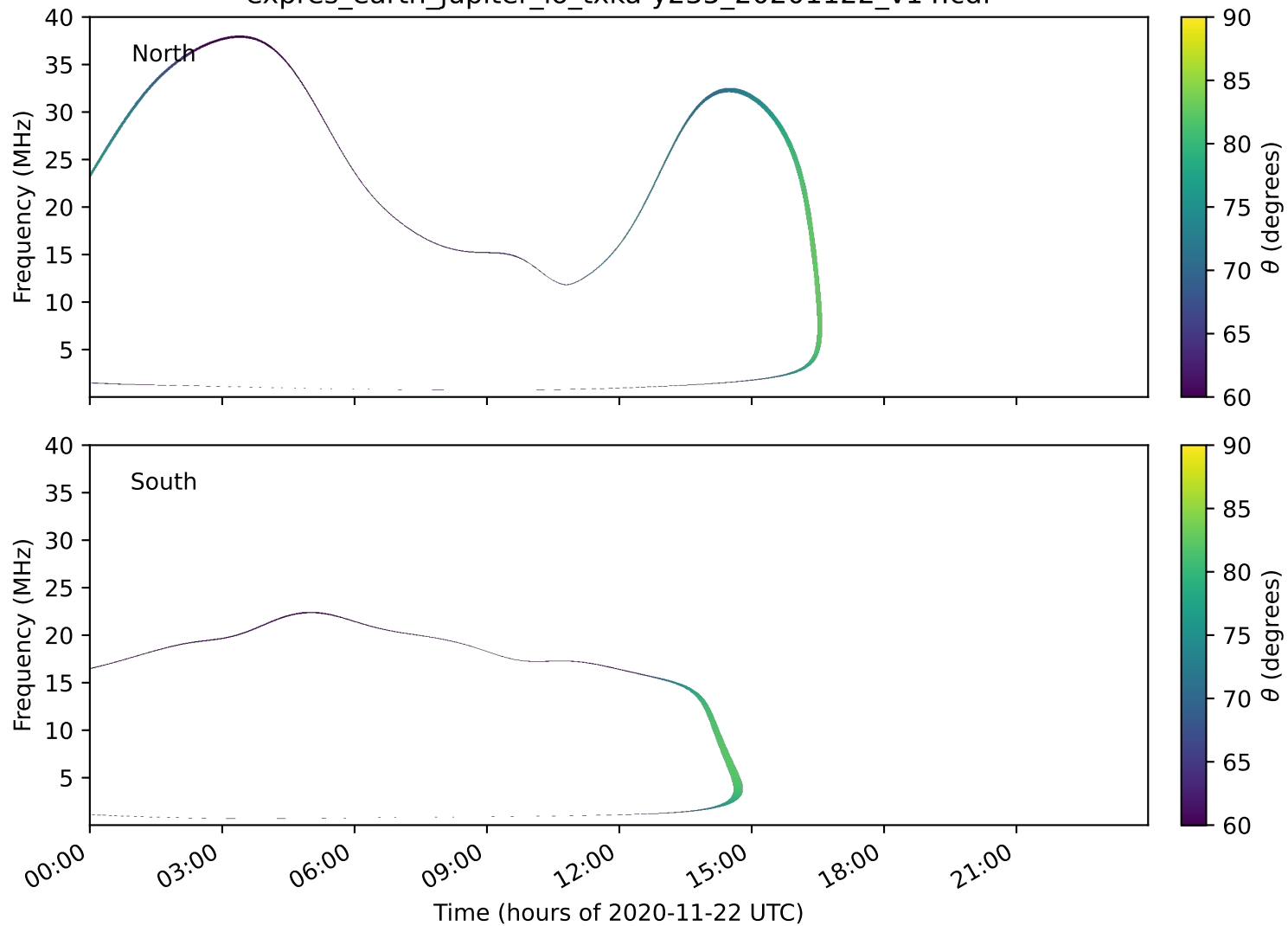
expres_earth_jupiter_io_txka-y235_20201122_v14.cdf
